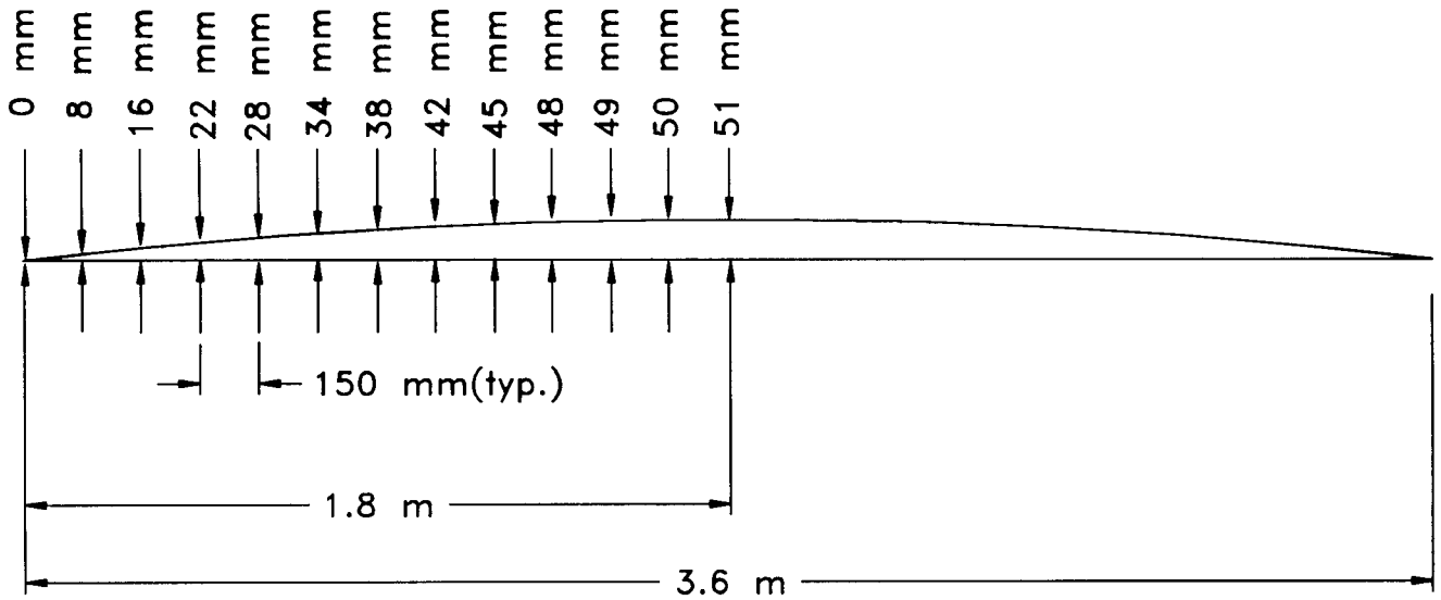
CROSS SECTION
